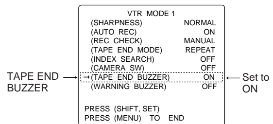
VTR mode 1 setting screen
